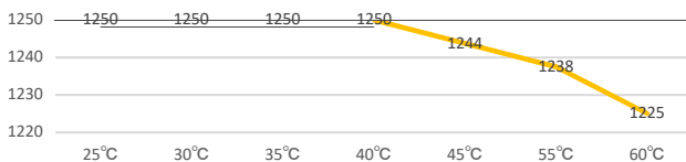
Temperature (CePEMius)Derate Curves Unit: kVA
